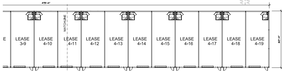
FLOOR PLAN -AREA A
