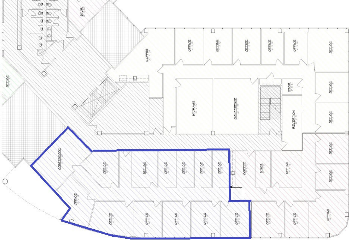
(A) 2ND FLOOR - FLOOR PLAN N.T.S.
